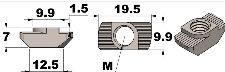
T-SLOT – 10 MM HAMMER NUTS
