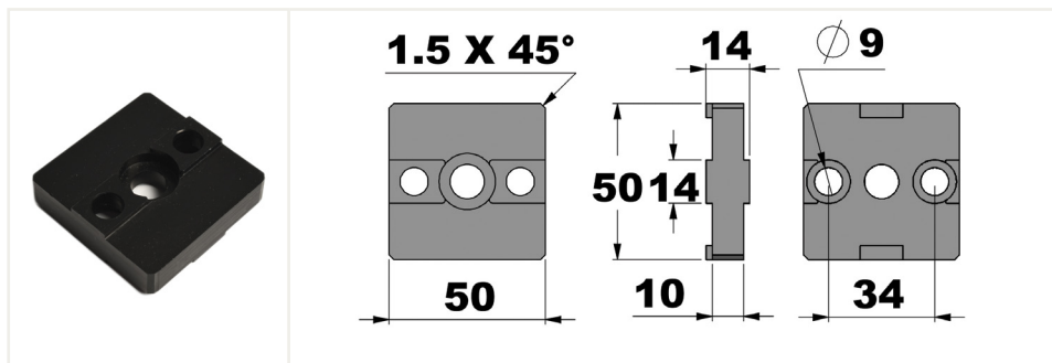
CONNECTOR FOR PROFILE 50X50 – SLOT 14
