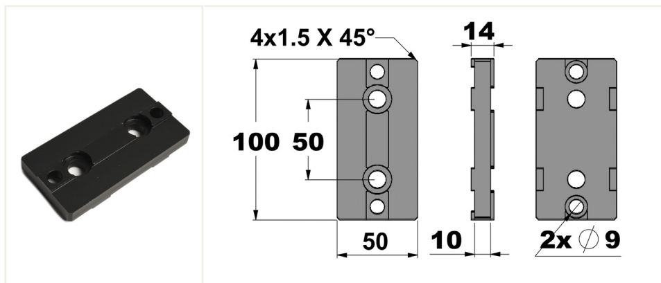
CONNECTOR FOR PROFILE 50X100 – SLOT 14
