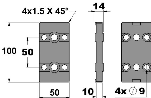
CONNECTOR FOR PROFILE 50X100 – SLOT 14
