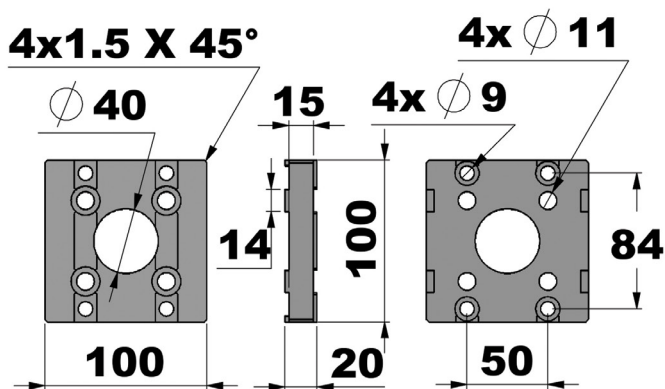
CONNECTOR FOR PROFILE 100X100 – SLOT 14
